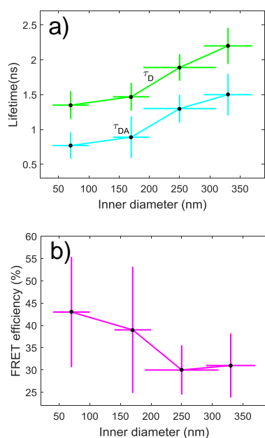
Figure 5. a) Lifetime measurements of site-selective functionalized plasmonic nanopores with single ATTO 520 and with ATTO 520 and ATTO 590 altogether. Each data point is the result of the measurement of two arrays of 49 nanopores (see Methods). The fluorescence from the ATTO 520 dyes has been measured in the 553–577 nm spectral band. b) Average FRET efficiency for the ATTO520-ATTO590 FRET pair. The FRET efficiency is computed with the relation \eta_{FRET} = 1 - \tau_{DA}/\tau_D with the data given in Figure 6a.
