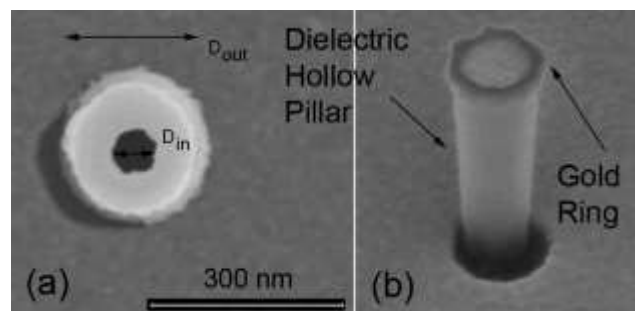
Figure 1: SEM images of the fabricated nanopores. (a) Nanoring prepared with 80pA ion current; (b) tilted view of the dielectric pillar and the metallic ring at the top. The thickness of the gold nanorings is 30nm (see Methods).
