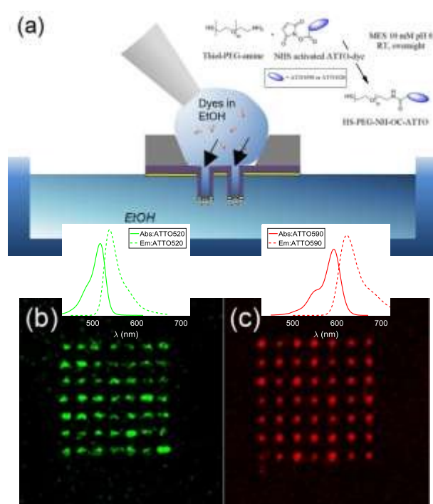
Figure 3: a) Sketch of the site-selective functionalization process. The nanopores are in contact with an EtOH bath. The other face of the sample is in contact with a solution of dyes in EtOH. The dyes diffuse through the channels and get attached to the nanopore thanks to the thiol group. Fluorescence images of plasmonic nanopores site-selectively decorated with ATTO dyes. b) The nanopores are functionalized with ATTO520. The laser excitation is at 488nm and the fluorescence detection at 500-550nm. c) The nanopores are functionalized with ATTO590. The laser excitation is at 561nm and the fluorescence detection at 570-620nm.
