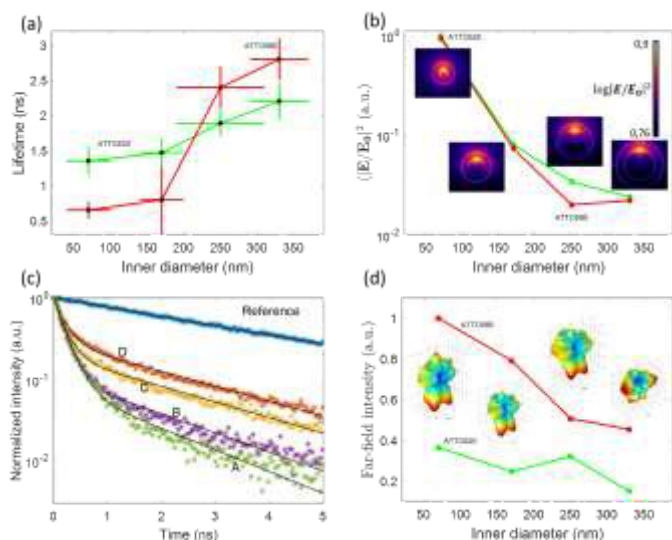
Figure 4. (a) Lifetime measurements of site-selective functionalized plasmonic nanopores with single ATTO 520 and ATTO 590 as a function of the inner diameter of the nanopore. Each data point is the result of the measurement of two arrays of 49 nanopores (see Methods). The fluorescence from the ATTO 520 (590) dyes has been measured in the 553-577 (593-643) nm spectral band. (b) Average intensity emitted by an electric dipole in the nanopore volume. The dipoles emit at 565nm and 618nm respectively. The insets are near-field distributions of the field induced by the dipole emitting at 565nm. (c) Representative lifetime measurements of the four nanopores, as well as the reference case. (d) Far-field intensity emitted by dipoles emitting at 565 nm and 618nm. The far-field is calculated on a horizontal plane on top of the nanopore. The insets are the far-field distributions induced by the emitting dipole at 618 nm.
