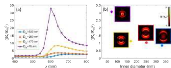
Figure 2. a) Spectra of the intensity enhancement for the four nanopores under a tightly focused Gaussian beam. b) Average field intensity enhancement for the four different fabricated nanopores calculated in the volume of the plasmonic ring. The simulations are done for a linearly polarized Gaussian beam that is tightly focused ( w_0 = 350 nm) at 532 nm. Insets: near-field profiles induced by the tightly focused Gaussian beam at 532 nm.
