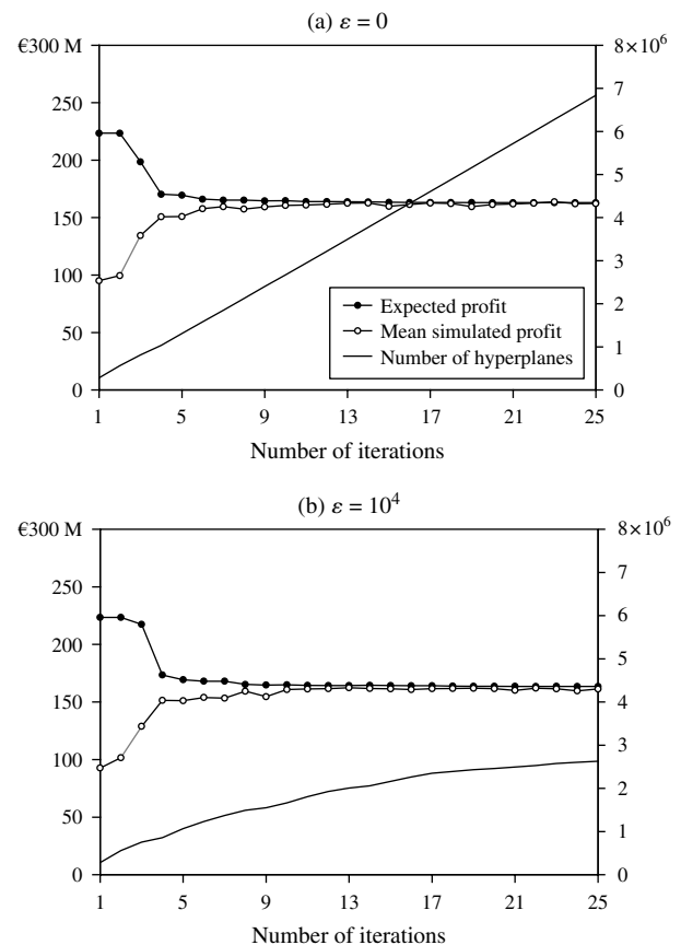
Figure 3. Convergence of ADPP for different approximation bounds for the case 50% min capacity.
