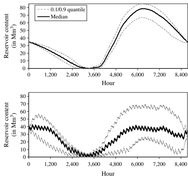
Figure 4. Reservoir content curves.
