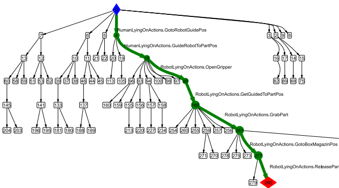
Fig. 8 This state space was created by the search algorithm also with the Automatic assistance selected, but through the fact that the part position is unknown, the solution consists of the actions of the Collaborative assistance behavior.
