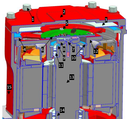
Fig. 4 A cross-sectional view of an electrical drive with numbered parts.
