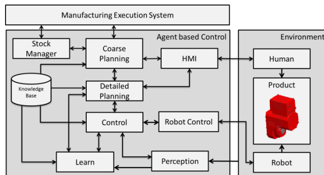
Fig. 1 The agent’s architecture and the information flow between the different software modules.
