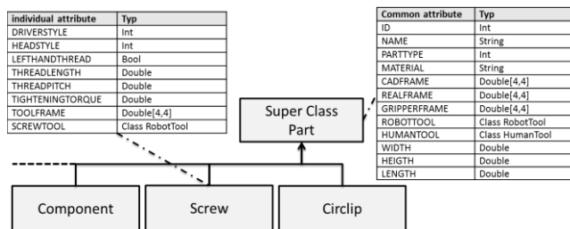
Fig. 2 The inheritance hierarchy of part classes with details of common and individual attributes.
