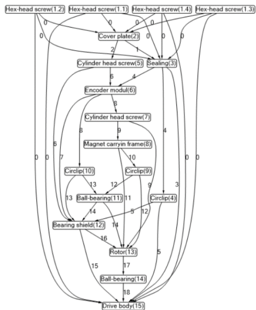
Fig. 5 A product graph of the electrical drive of Figure 4. The numbers on the edges are the IDs of connection instances.
