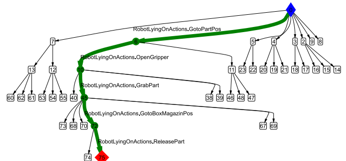
Fig. 7 A state space created by the search algorithm. From the initial state (blue diamond) and with the Automatic assistance behavior, a solution state (red diamond) was found, and the robot actions on the green path could be executed.
