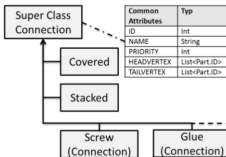
Fig. 3 Inheritance hierarchy of the connection class. The ordering implied the disassembly priority of each class from low to high. Also illustrated are the common attributes of the super class.
