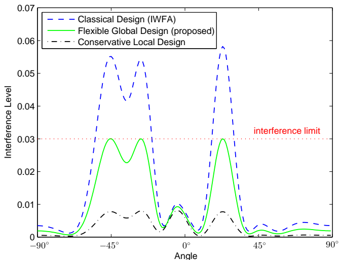
Figure 1. Typical interference profile at a PU as a function of the angle caused by the SUs in a MIMO CR system, under local (black curve), global (green curve), and no (blue curve) interference constraints.
