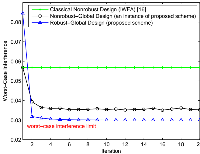
Figure 2. Worst-case interference \sum_{i=1}^I t_{pi}^*(\mu^\nu) versus iteration number \nu in Algorithm 1 for robust and nonrobust formulation.
