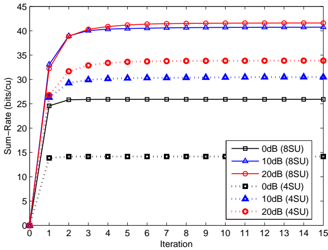
Figure 4. Convergence of Algorithm 3: Sum-rate of all SUs \sum_{i=1}^I r_i(\mathbf{Q}^\nu) versus iteration number \nu with \mathbf{Q}_i^0 = \mathbf{0} for all i = 1, \dots, I .
