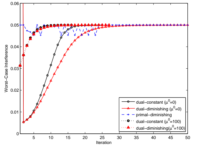
Figure 5. Worst-case aggregate interference at the PU: \sum_{i=1}^I t_{pi}^*(\boldsymbol{\mu}^n; \mathbf{Q}^\nu) in the dual-based Algorithm 5 and \sum_{i=1}^I \kappa_{pi}^n(\mathbf{Q}^\nu) in the primal-based Algorithm 6 versus iteration number n for a given \mathbf{Q}^\nu .
