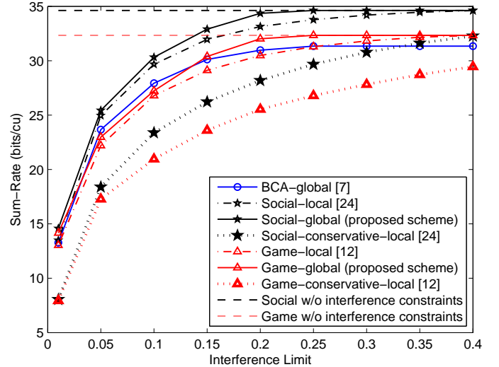
Figure 3. Sum-rate of all SUs \sum_{i=1}^I r_i(\mathbf{Q}) at a NE/socially optimal solution versus interference limit I^{\max} .
