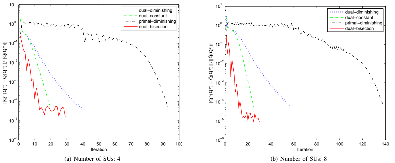
Figure 6. Convergence of dual-based Algorithm 5 and primal-based Algorithm 6: \|\mathbf{Q}^n(\mathbf{Q}^\nu) - \hat{\mathbf{Q}}(\mathbf{Q}^\nu)\|/\|\hat{\mathbf{Q}}(\mathbf{Q}^\nu)\| versus iteration number n for a given \mathbf{Q}^\nu , where \mathbf{Q}^n(\mathbf{Q}^\nu) \triangleq \mathbf{Q}^*(\mu^n; \mathbf{Q}^\nu) in Algorithm 5 and \mathbf{Q}^n(\mathbf{Q}^\nu) \triangleq \mathbf{Q}^*(\kappa^n; \mathbf{Q}^\nu) in Algorithm 6, and \hat{\mathbf{Q}}(\mathbf{Q}^\nu) is defined in (28).
