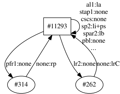
Figure 2. State #11293 is the start state. The transitions are annotated with input:output symbols. The ... indicate 30 more input-output pairs on the transition. The model overgeneralizes by merging states together despite low evidence of similarity.
