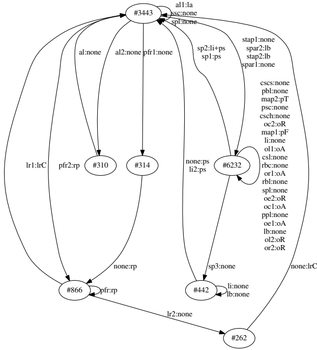
Figure 1. The original and fully recovered model of our example use case. State #3443 is the start state. The transitions are annotated with input:output symbols.
