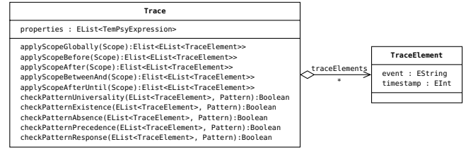
Fig. 1. Meta-model for execution traces
