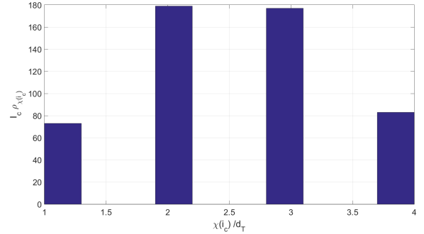
Fig. 9. Gaussian discrete PDF for \mathcal{I}_c = 512 chirps.
