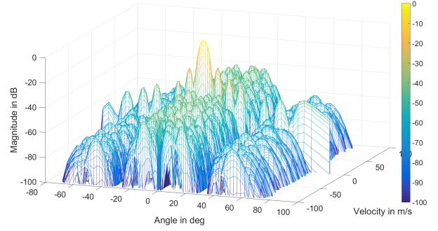
Fig. 3. Angle-Doppler AF for single target with SNR = 10 \text{ dB} , \mathcal{I}_c = 512 and uniform PDF
