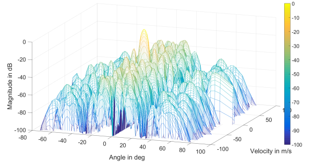
Fig. 5. Angle-Doppler AF for single target with SNR = 10 \text{ dB} , \mathcal{I}_c = 128 and rectangular PDF.
