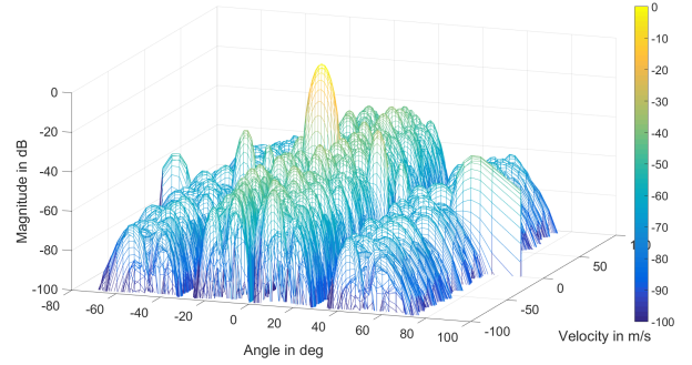
Fig. 4. Angle-Doppler AF for single target with SNR = 10 \text{ dB} , \mathcal{I}_c = 512 and Gaussian PDF.
