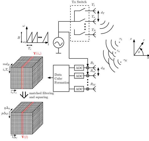
Fig. 1. FMCW System Diagram for white PCM modulation. The matrix \tilde{\mathbf{Y}} denotes the angle-Doppler ambiguity function for a particular range bin.
