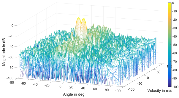
Fig. 7. Angle-Doppler AF for two target with SNR = -20 dB, \mathcal{I}_c = 512 and uniform PDF.
