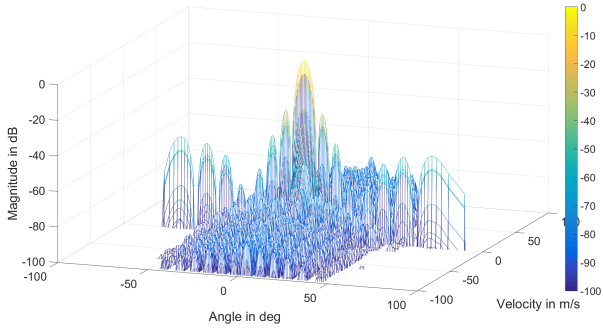
Fig. 6. Angle-Doppler AF for single target with SNR = 10 dB and \mathcal{I}_c = 512 using one transmitter and 16 receiver by applying conventional beamforming.
