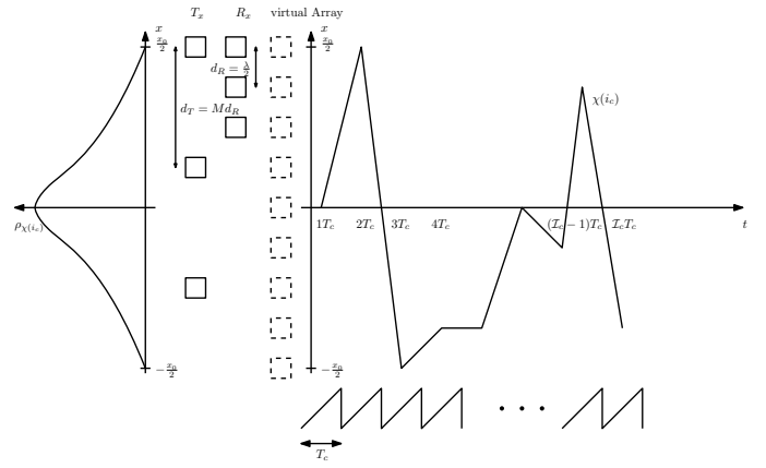
Fig. 2. Random PCM properties with the PCM PDF on left side and the uncorrelated phase center positions at the right side.
