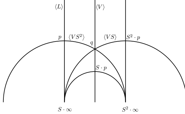
Figure 4: Geodesics fixed by certain finite order elements of \mathrm{PSL}_2(\mathbb{Z}[\sqrt{-1}]) .
