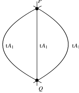
Figure 2: Two singular points P, Q which are analytically isomorphic to the singularity at the origin of \mathbb{C}^3/\mathcal{D}_2 .
