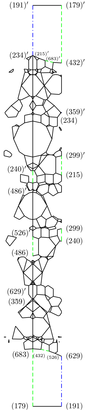
Figure 9: Fundamental domain in the case m = 191 . The coordinates of the vertices can be displayed by [35].
