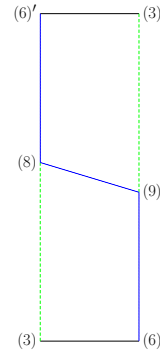
Figure 8: Fundamental domain in the case m = 11 .
