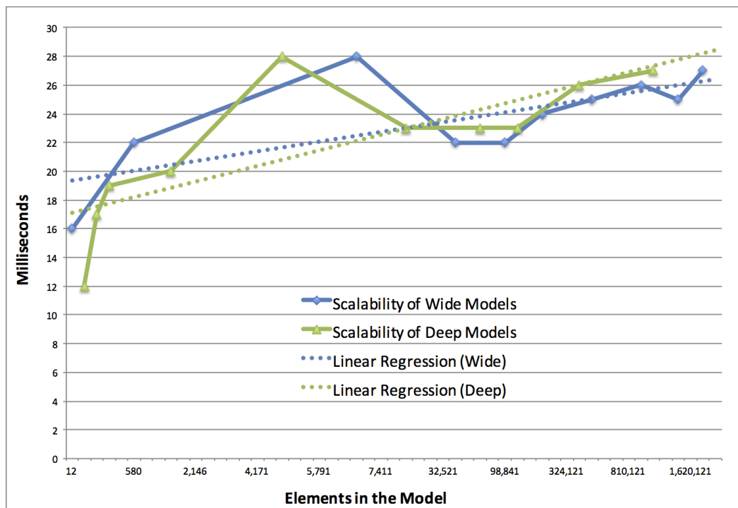
Figure 6.5: Scalability of read operations for large-scale models
