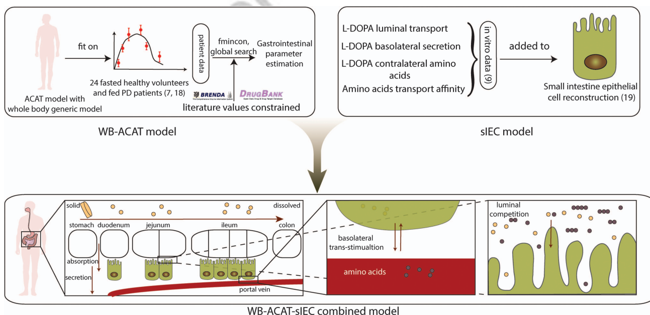
Figure 1. The multiscale PBPK-COBRA model used in this study. We combined a spatially and dynamically refined PBPK model (deemed WB-ACAT) of the gastrointestinal tract with seven copies of a mechanistically accurate and detailed metabolic model of small intestinal epithelial cells (sIEC). COBRA, constraint-based reconstruction and analysis; PBPK, physiologically based pharmacokinetic; WB-ACAT, whole-body advanced compartmental absorption and transit.
