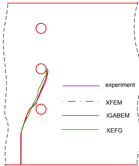
FIGURE 2.18: Crack paths (XEFG result \Delta a = 0.1 is from Ventura et al , 2002)
