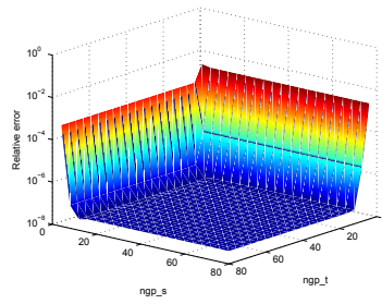
(b) mesh B with \omega = 0.1
