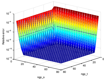
(c) mesh C with \omega = 0.1
