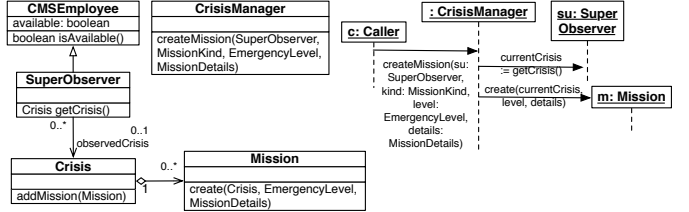
Fig. 3. A partial design of CMS with createMission function [6]
