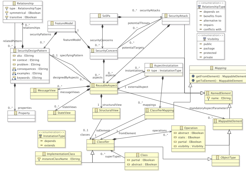
Fig. 4. Meta-model of System of Security design Patterns (SoSpa-MM)
