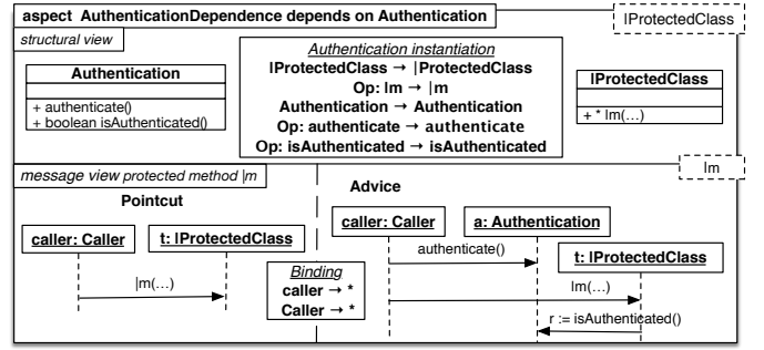
Fig. 11. Aspect AuthenticationDependence (renamed to L1 in Fig. 5)
