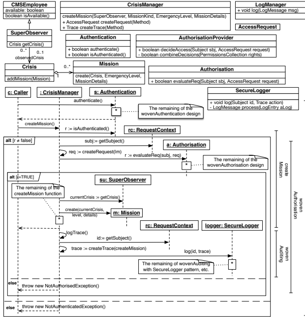
Fig. 15. Automatically Woven Secure CMS Model
