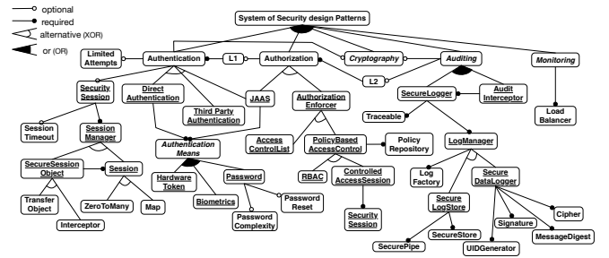
Fig. 5. A partial feature model of SoSpa
