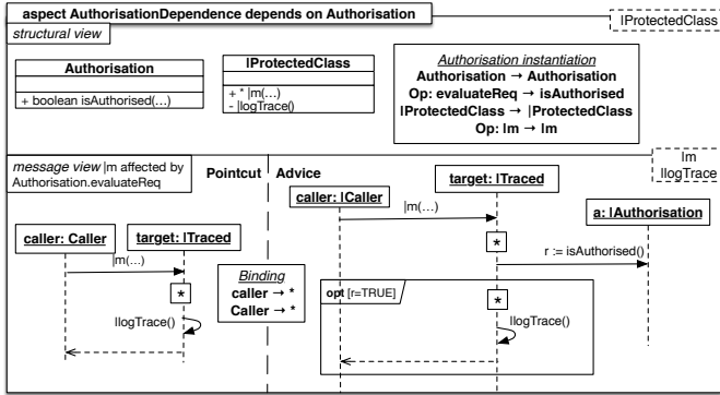
Fig. 14. Aspect AuthorisationDependence (renamed to L2 in Fig. 5)
