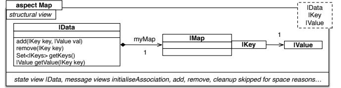
Fig. 2. Aspect Map (partially)
