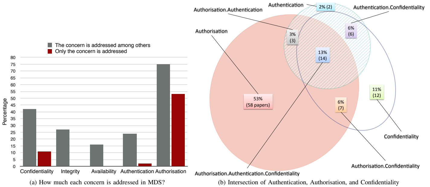
Fig. 6: Statistics of Security Concerns addressed by the reviewed MDS studies
