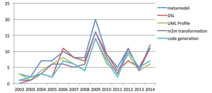
Fig. 10: Trend of MDE artefacts leveraged by MDS studies
