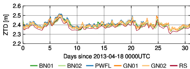
Fig. 3 RT-PPP ZTD estimates and RS-based ZTD for station HERT
