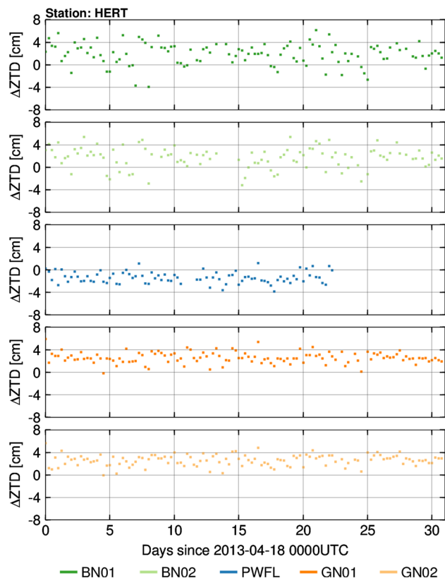
Fig. 4 Difference of RT-PPP ZTD and RS-based ZTD estimates for station HERT
