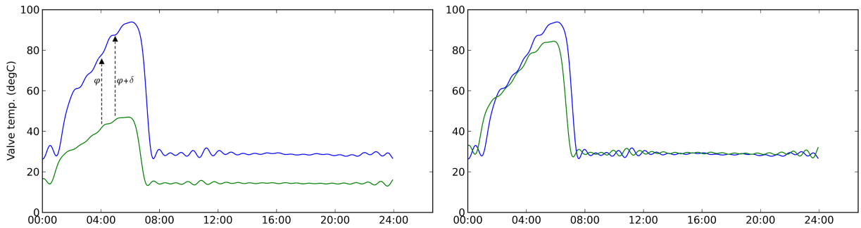
Figure 2: Fourier series representation of two thermal signatures f_1 (lower curve) and f_2 (upper curve). We apply the affine transforms on the f_1 curve to obtain f_1' , which appears on the plot on right hand side. The algorithm evaluated the best fit with a = 0.502 and k = 0.21 , using the points at 180^\circ and 190^\circ .
