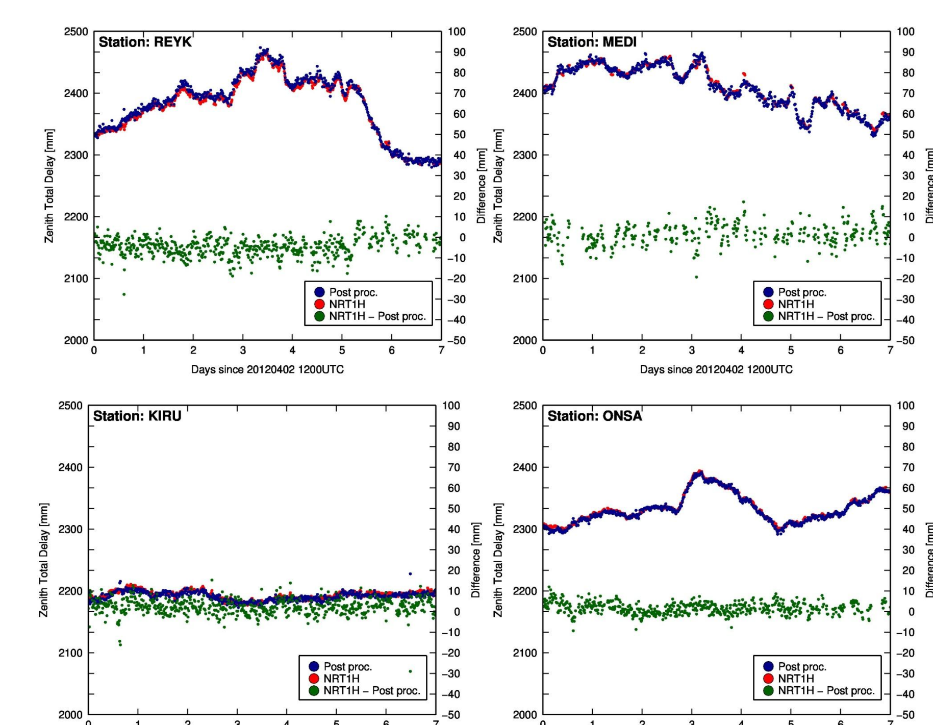
Figure 3: Comparison of ZTD time series obtained from NRT1H and post-processed solution for 4 stations for 2012-04-02 12:00UTC to 2012-04-09 12:00UTC (Note the different scales for the estimates and the difference)
