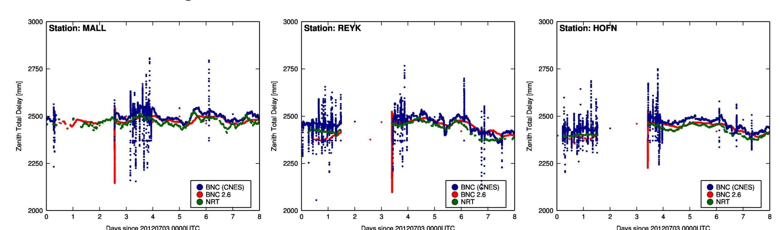
Figure 7: ZTD time-series obtained from CNES BNC (blue), BNC v2.6 (red) and near real-time system (green) for three stations for 2012-07-03 00:00UTC to 2012-07-11 00:00UTC
