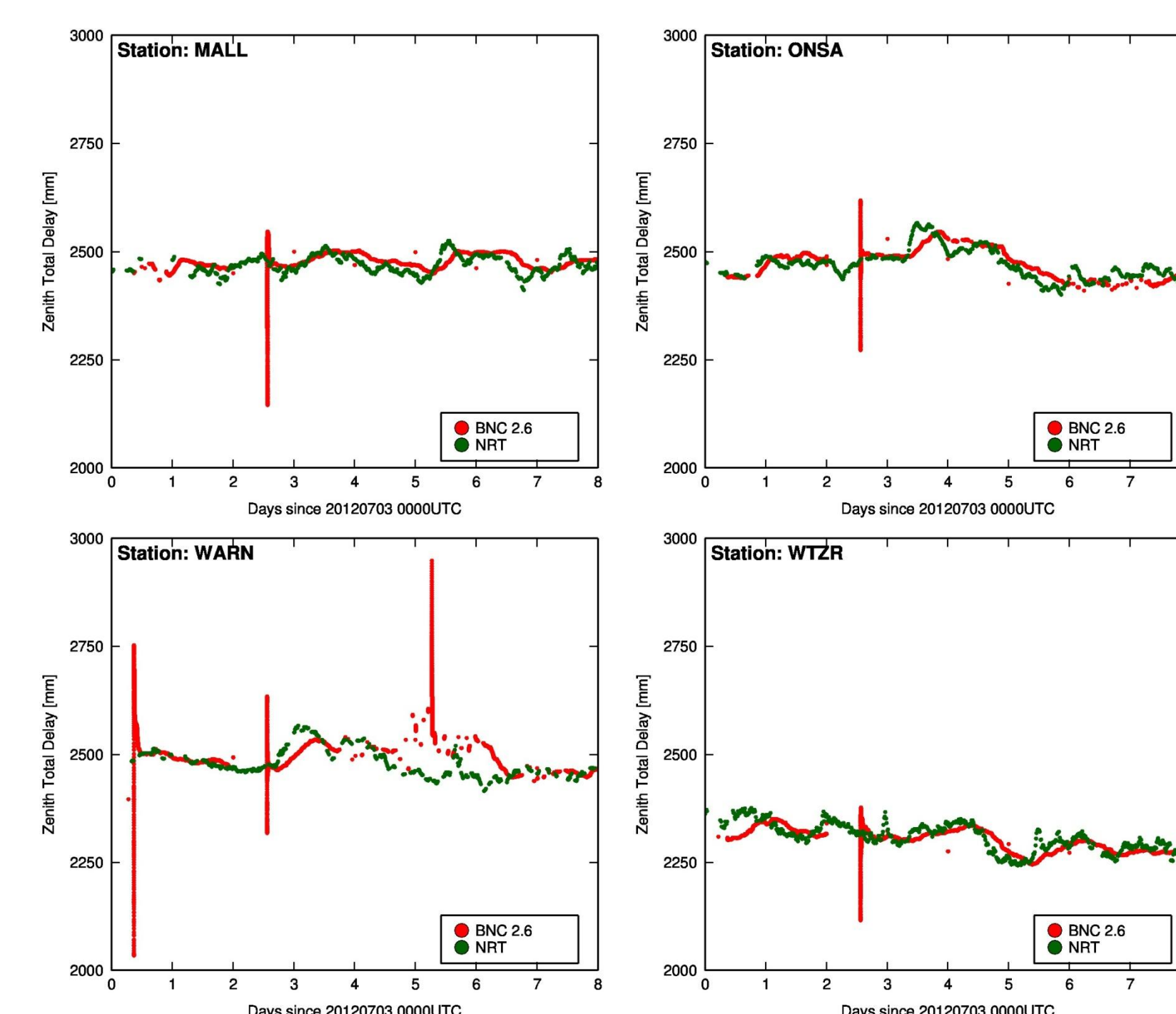
Figure 5: Comparison of ZTD time-series obtained in real-time and near real-time for 4 stations for 2012-07-03 00:00UTC to 2012-07-11 00:00UTC
