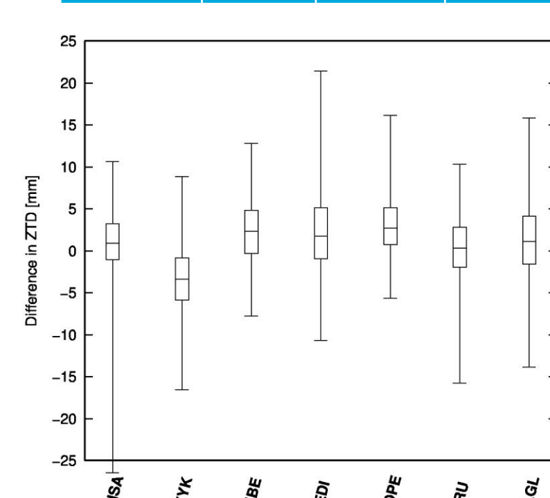
Figure 2: Box-and-Whisker plot showing statistics for the comparison between NRT1H and IGS Final Troposphere product
