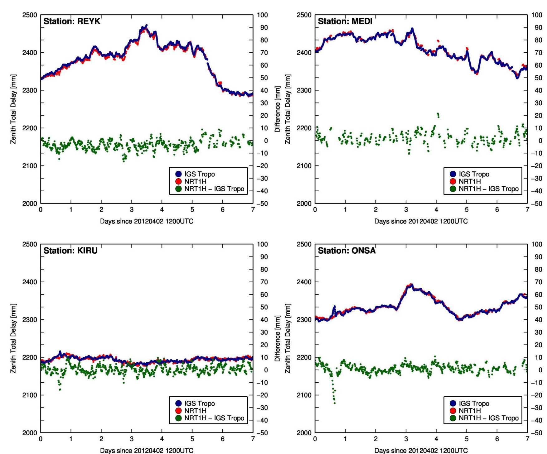
Figure 1: Comparison of ZTD time series obtained from NRT1H and IGS Final Troposphere product for 4 stations for 2012-04-02 12:00UTC to 2012-04-09 12:00UTC (Note the different scales for the estimates and the difference)
